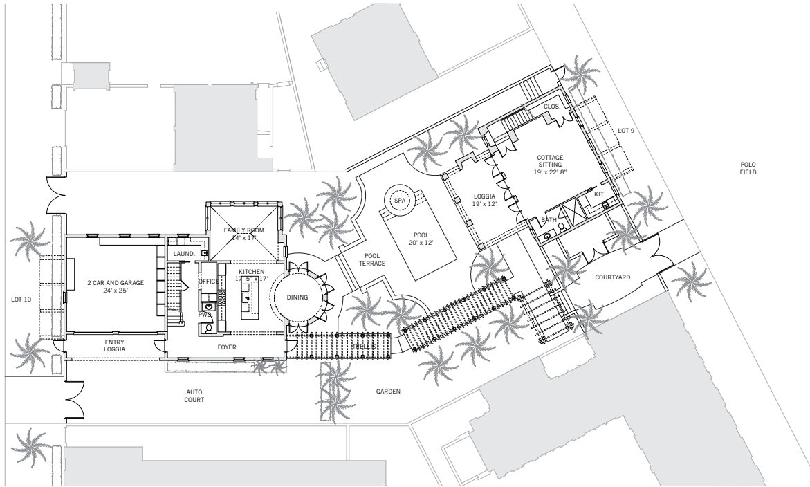
GROUND FLOOR
