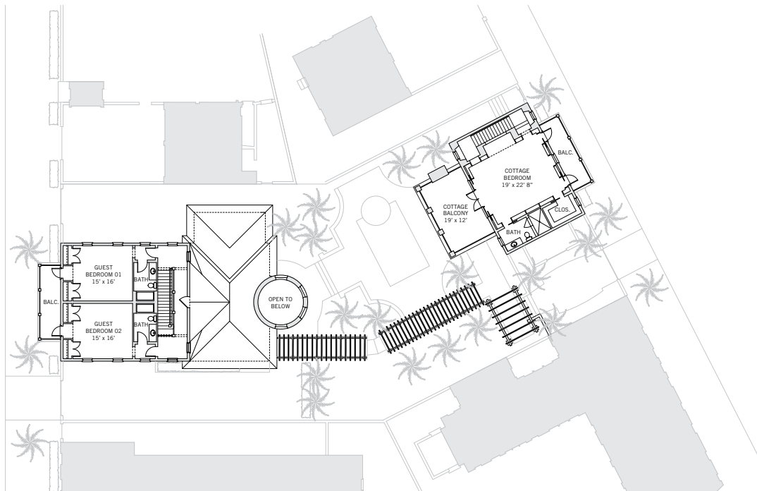
SECOND FLOOR
