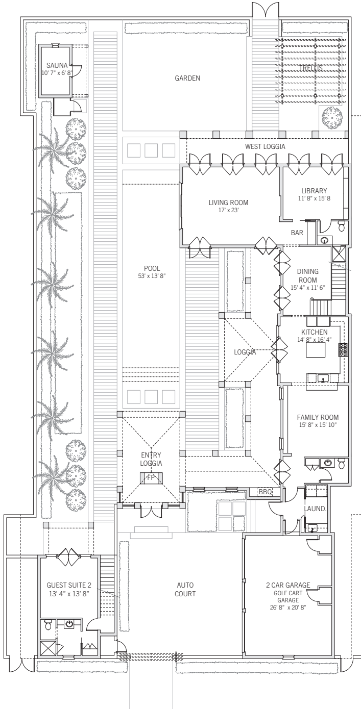
GROUND FLOOR
